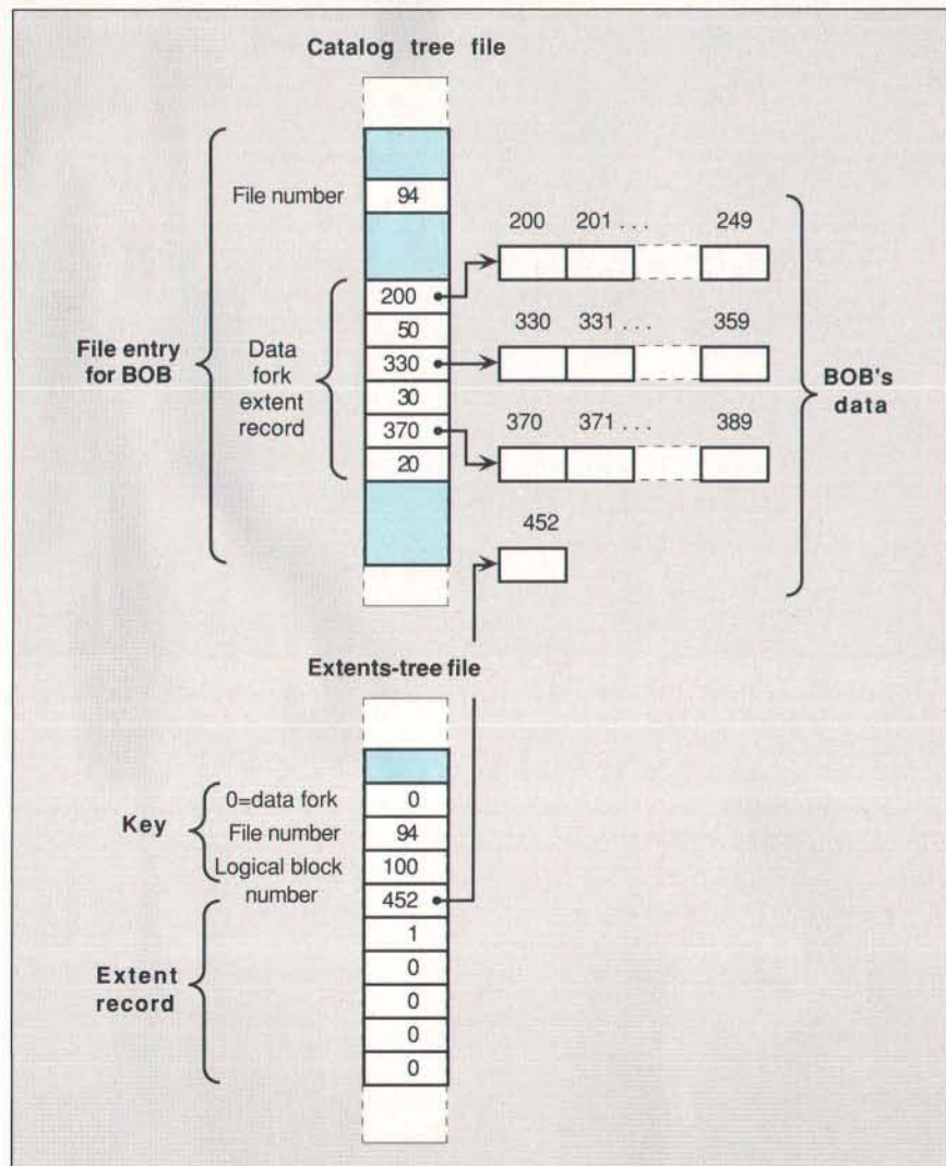
Figure 4: The file BOB is stored on the HFS volume. The file's data fork has become so fragmented that the system has had to create an extents-tree entry.
